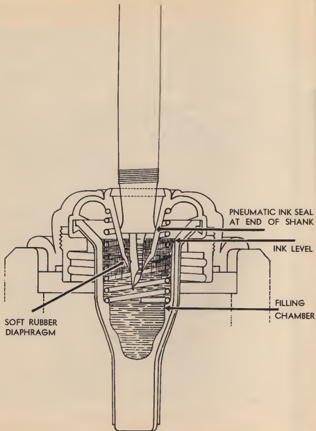
FIRST — Pen Seated in Penfiller.
